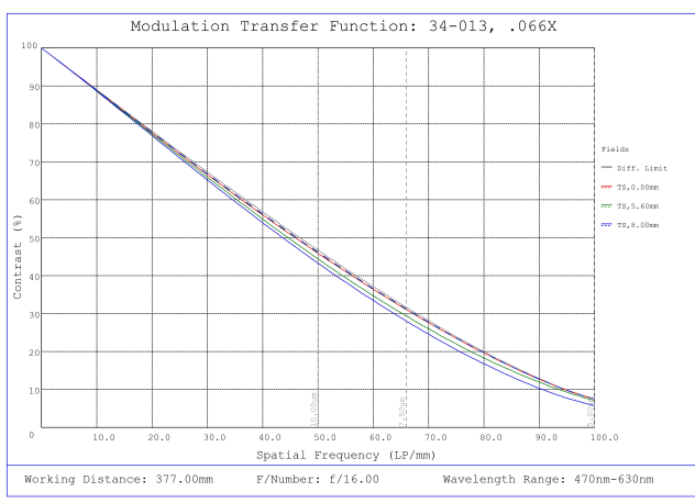
#34-013, 0.066X, 1" C-Mount TitanTL® Telecentric Lens, Modulated Transfer Function (MTF) Plot, 377mm Working Distance, f16
