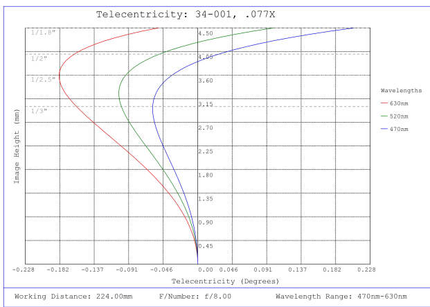
#34-001, 0.077X, 1/1.8" C-Mount TitanTL® Telecentric Lens, Telecentricity Plot
