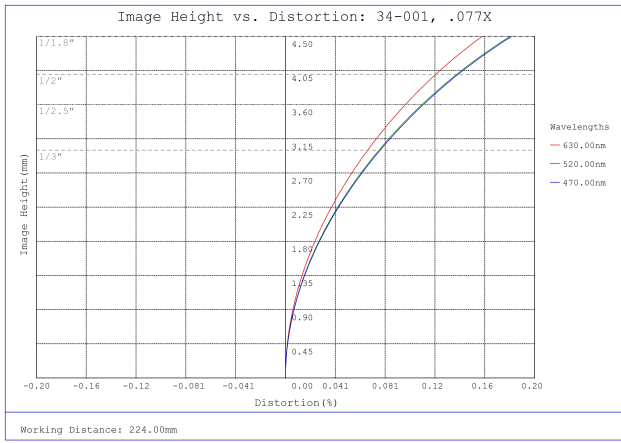
#34-001, 0.077X, 1/1.8" C-Mount TitanTL® Telecentric Lens, Distortion Plot
