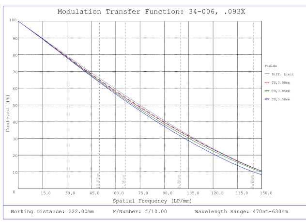
#34-006, 0.093X, 2/3" C-Mount TitanTL® Telecentric Lens, Modulated Transfer Function (MTF) Plot, 222mm Working Distance, f10
