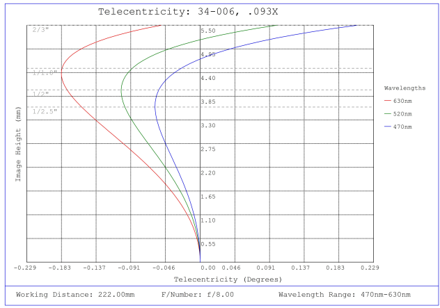
#34-006, 0.093X, 2/3" C-Mount TitanTL® Telecentric Lens, Telecentricity Plot
