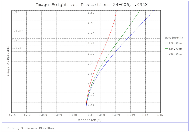
#34-006, 0.093X, 2/3" C-Mount TitanTL® Telecentric Lens, Distortion Plot
