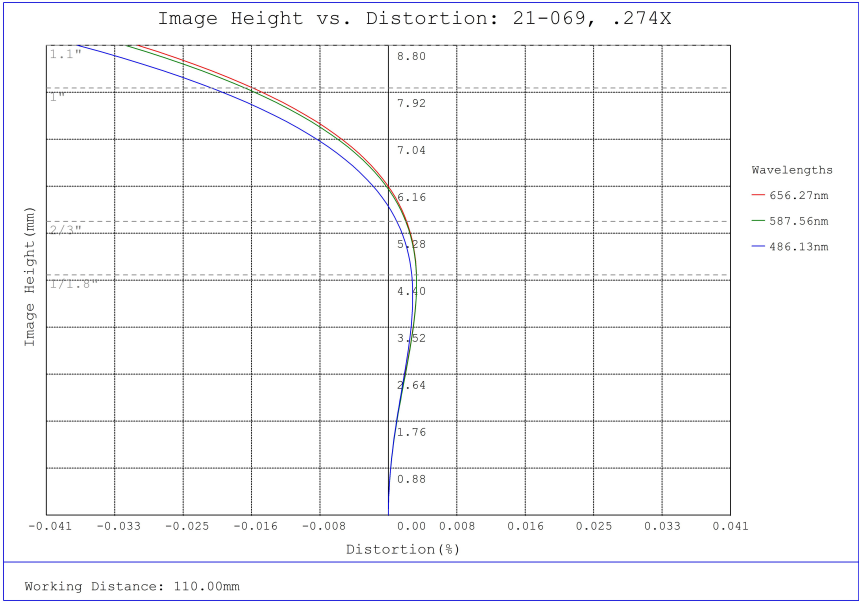
#21-069, 0.274X In-Line CobaltTL Telecentric Lens, Distortion Plot
