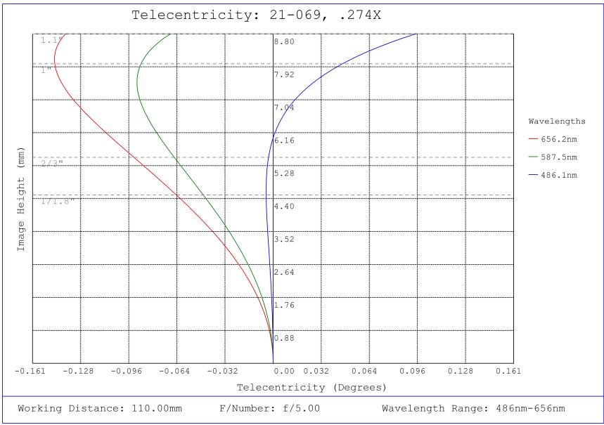
#21-069, 0.274X In-Line CobaltTL Telecentric Lens, Telecentricity Plot
