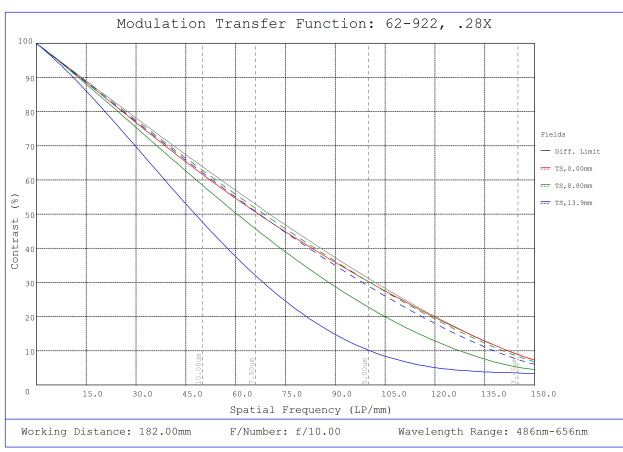
#62-922, 0.28X, 28.7mm F-Mount PlatinumTL™ Telecentric Lens, Modulated Transfer Function (MTF) Plot, 182mm Working Distance, f10
