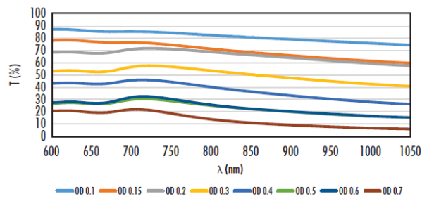
NIR I Coated HOYA ND Filters
