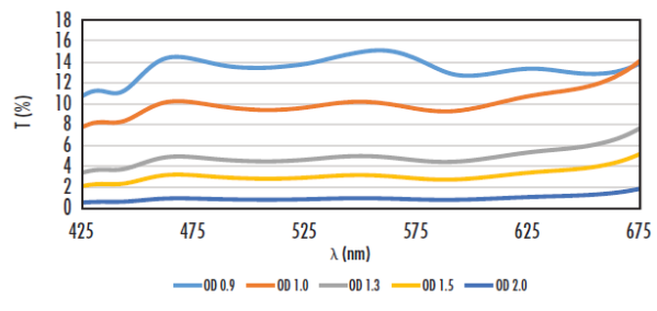
VIS 0° Coated HOYA ND Filters
