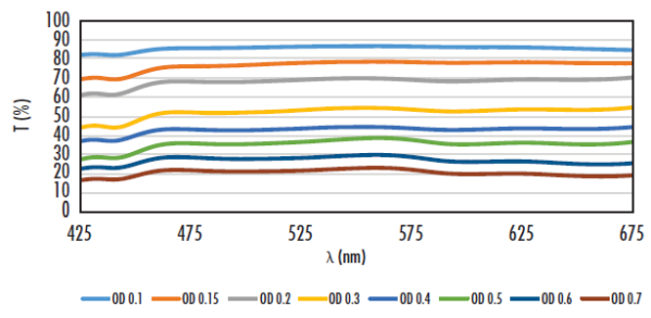
VIS 0° Coated HOYA ND Filters
