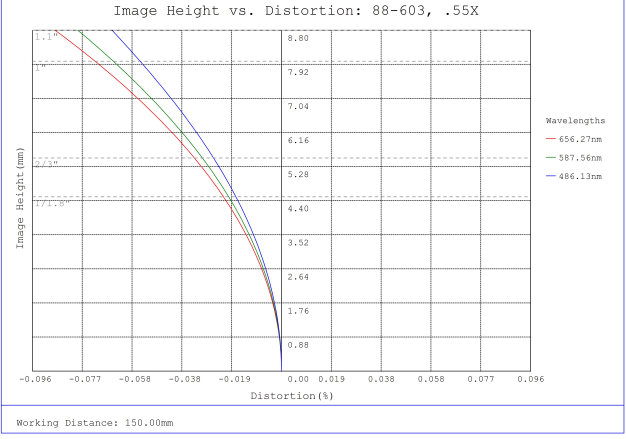
#88-603, 0.55X CobaltTL Telecentric Lens, Distortion Plot
