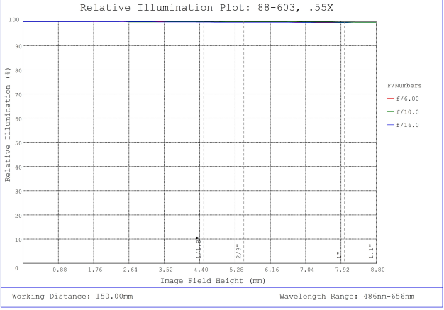
#88-603, 0.55X CobaltTL Telecentric Lens, Relative Illumination Plot
