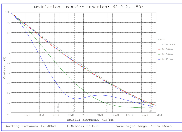
#62-912, 0.5X, 28.7mm F-Mount PlatinumTL™ Telecentric Lens, Modulated Transfer Function (MTF) Plot, 175mm Working Distance, f10
