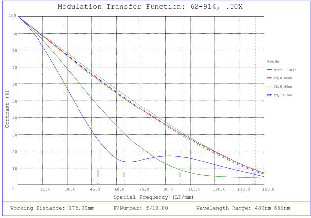
#62-914, 0.5X, 28.7mm M42 x 1.0 (19.53mm) PlatinumTL™ Telecentric Lens, Modulated Transfer Function (MTF) Plot, 175mm Working Distance, f10
