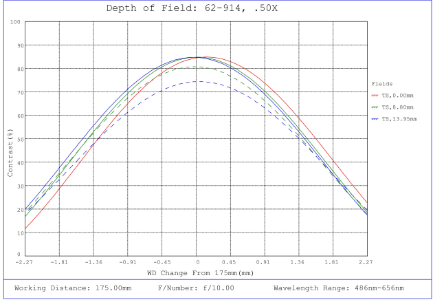
#62-914, 0.5X, 28.7mm M42 x 1.0 (19.53mm) PlatinumTL™ Telecentric Lens, Depth of Field Plot, 175mm Working Distance, f10
