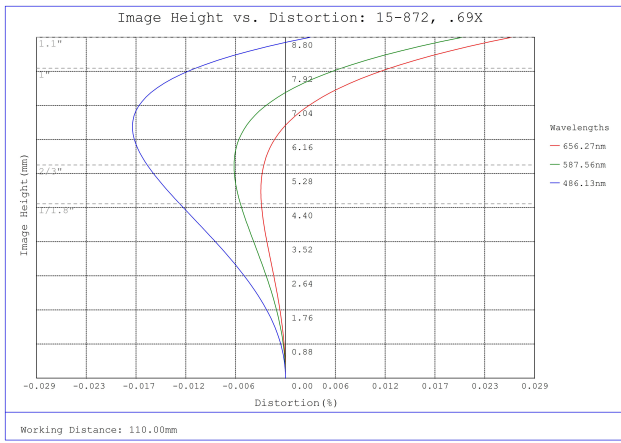
#15-872, 0.69X CobaltTL Telecentric Lens, Distortion Plot
