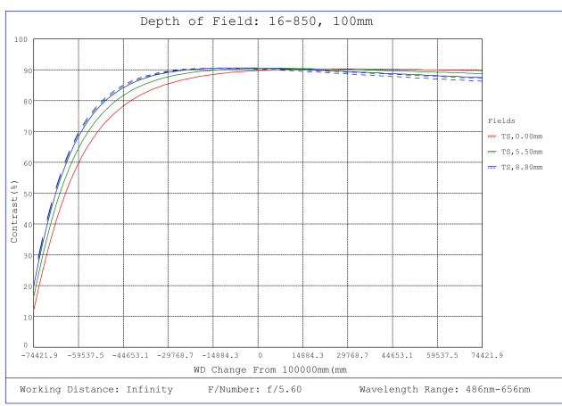
#16-850, 100mm, f/5.6 Athermal Lens, Depth of Field Plot, 10000mm Working Distance, f5.6
