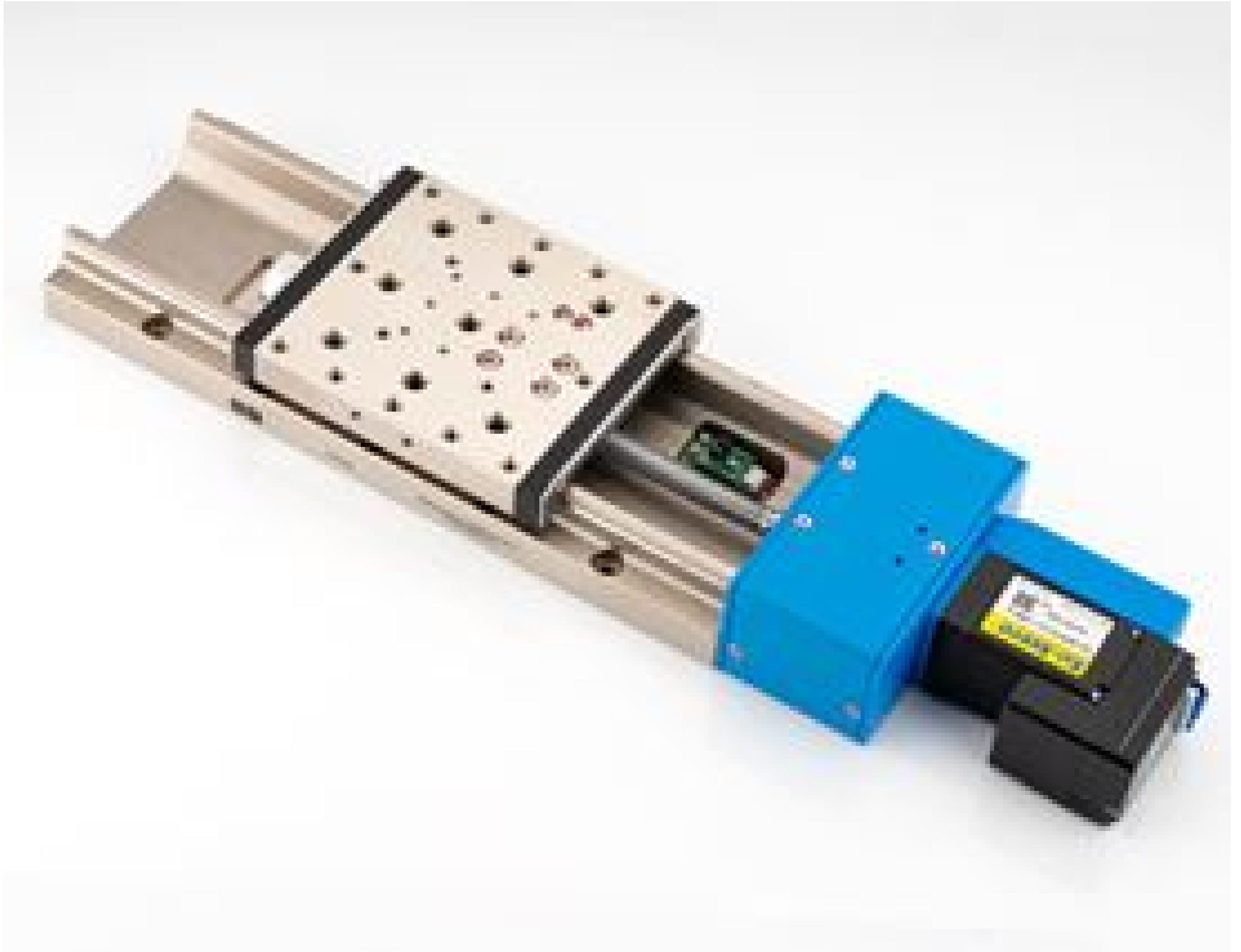
100mm Travel, 80mm Square TECHSPEC Motorized Linear Stage, Metric
