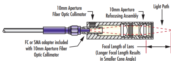
Fiber with 10mm Aperture Fiber Optic Collimator and Refocusing Assembly
