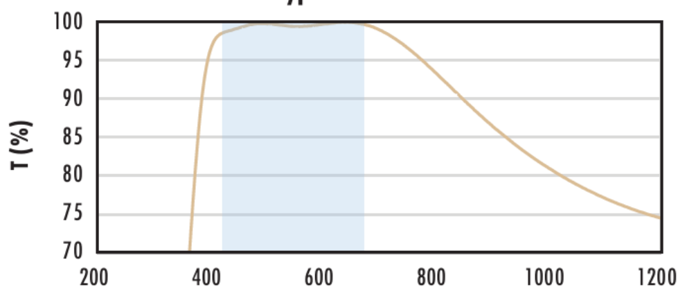
N-BK7 with VIS 0° Coating Typical Transmission
