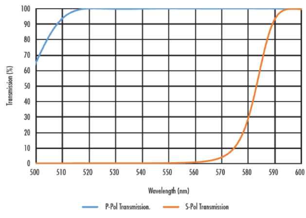
532nm Polarizing Cube Beamsplitter
