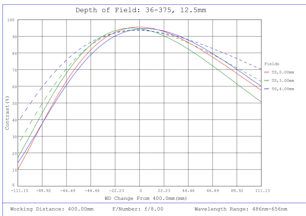
#36-375, 12.5mm FL f/8, Rugged Blue Series M12 Lens, Depth of Field Plot, 400mm Working Distance, f8
