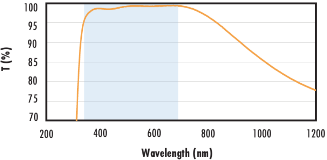
Fused Silica with VIS-EXT Coating Typical Transmission
