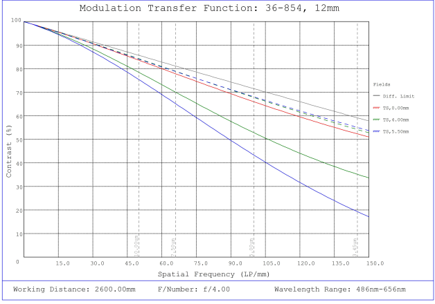
#36-854, 12mm f/4, 1000mm-∞ Primary WD, HRr Series Fixed Focal Length Lens, Modulated Transfer Function (MTF) Plot, 2600mm Working Distance, f4
