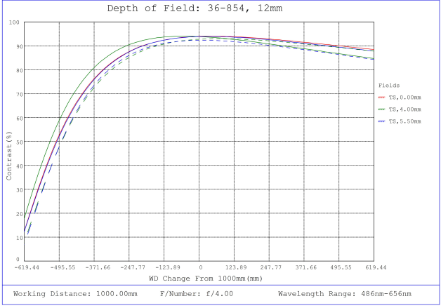
#36-854, 12mm f/4, 1000mm-∞ Primary WD, HRr Series Fixed Focal Length Lens, Depth of Field Plot, 1000mm Working Distance, f4
