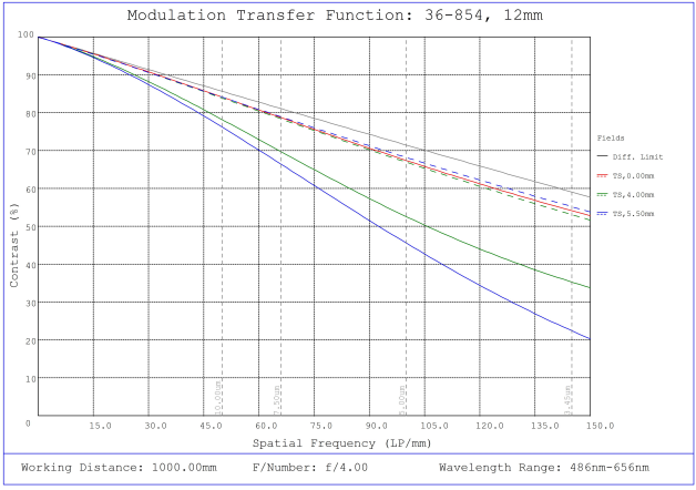
#36-854, 12mm f/4, 1000mm-∞ Primary WD, HRr Series Fixed Focal Length Lens, Modulated Transfer Function (MTF) Plot, 1000mm Working Distance, f4
