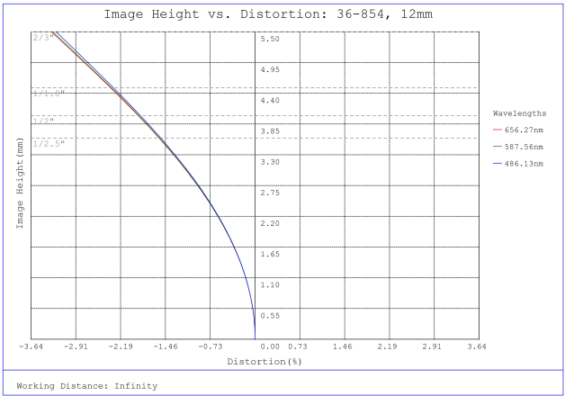
#36-854, 12mm f/4, 1000mm-∞ Primary WD, HRr Series Fixed Focal Length Lens, Distortion Plot
