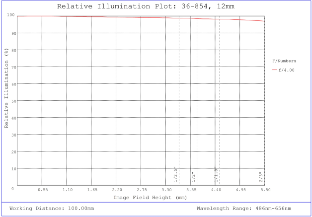
#36-854, 12mm f/4, 1000mm-∞ Primary WD, HRr Series Fixed Focal Length Lens, Relative Illumination Plot
