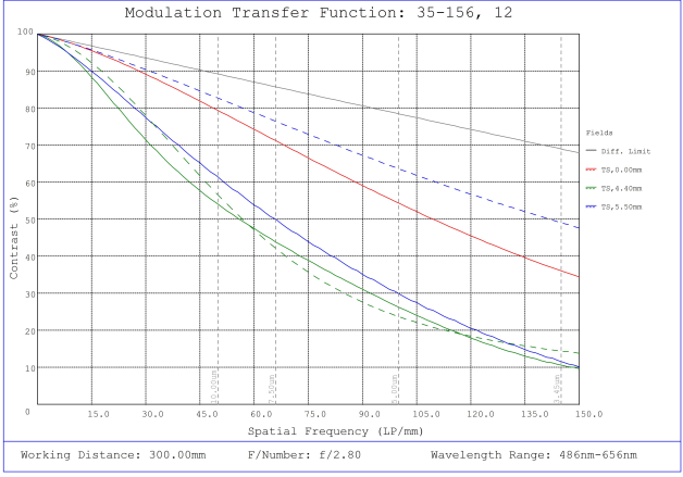
#35-156, 12mm, f/2.8 Cr Series Fixed Focal Length Lens, Modulated Transfer Function (MTF) Plot, 300mm Working Distance, f2.8
