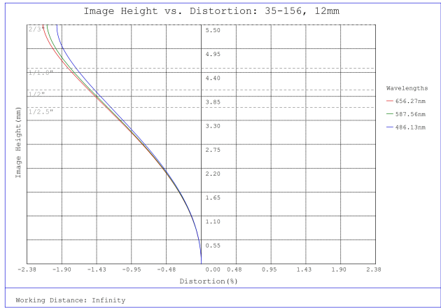
#35-156, 12mm, f/2.8 Cr Series Fixed Focal Length Lens, Distortion Plot
