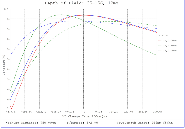
#35-156, 12mm, f/2.8 Cr Series Fixed Focal Length Lens, Depth of Field Plot, 750mm Working Distance, f2.8
