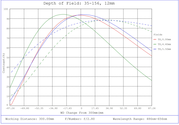
#35-156, 12mm, f/2.8 Cr Series Fixed Focal Length Lens, Depth of Field Plot, 300mm Working Distance, f2.8
