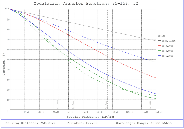
#35-156, 12mm, f/2.8 Cr Series Fixed Focal Length Lens, Modulated Transfer Function (MTF) Plot, 750mm Working Distance, f2.8
