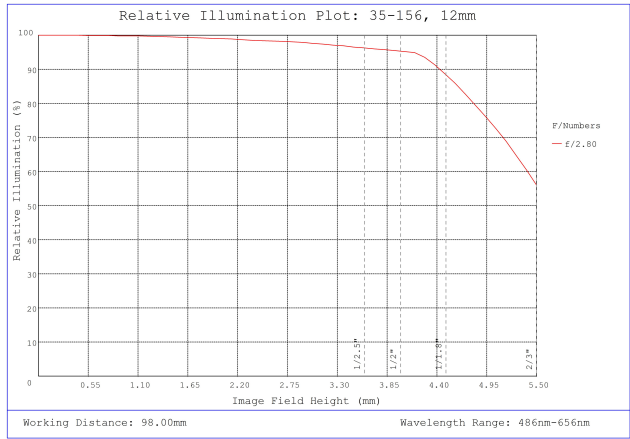
#35-156, 12mm, f/2.8 Cr Series Fixed Focal Length Lens, Relative Illumination Plot
