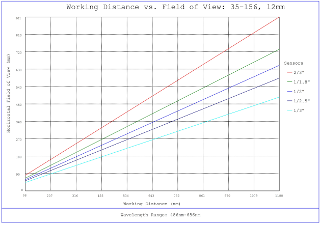
#35-156, 12mm, f/2.8 Cr Series Fixed Focal Length Lens, Working Distance versus Field of View Plot
