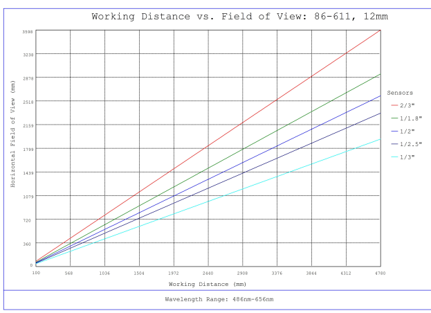
#86-611, 12mm, f/8 Ci Series Fixed Focal Length Lens, Working Distance versus Field of View Plot
