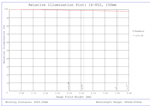
#16-852, 150mm, f/4 Athermal Lens, Relative Illumination Plot
