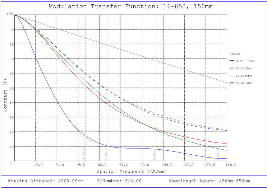
#16-852, 150mm, f/4 Athermal Lens, Modulated Transfer Function (MTF) Plot, 4000mm Working Distance, f4
