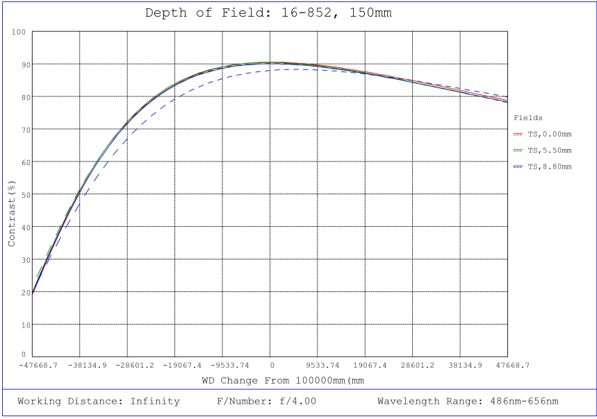
#16-852, 150mm, f/4 Athermal Lens, Depth of Field Plot, 100000mm Working Distance, f4
