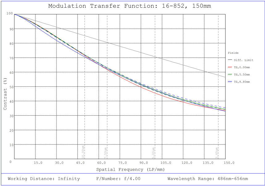
#16-852, 150mm, f/4 Athermal Lens, Modulated Transfer Function (MTF) Plot, Working Distance: Infinity, f4
