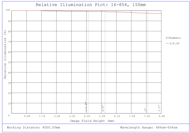
#16-854, 150mm, f/8 Athermal Lens, Relative Illumination Plot
