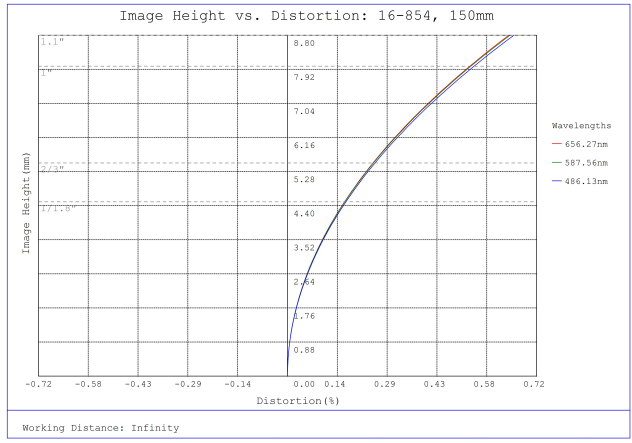
#16-854, 150mm, f/8 Athermal Lens, Distortion Plot
