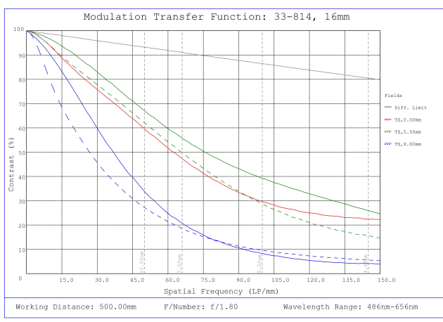
#33-814, 16mm f/1.8, HPI Series Fixed Focal Length Lens, Modulated Transfer Function (MTF) Plot, 500mm Working Distance, f1.8
