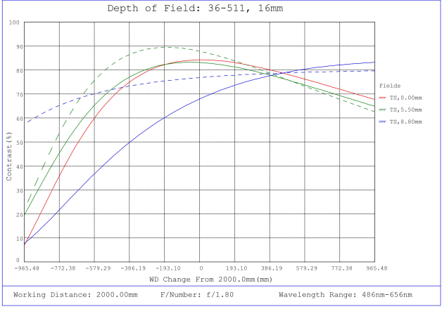
#36-511, 16mm f/1.8, HPr Series Fixed Focal Length Lens, Depth of Field Plot, 2000mm Working Distance, f1.8
