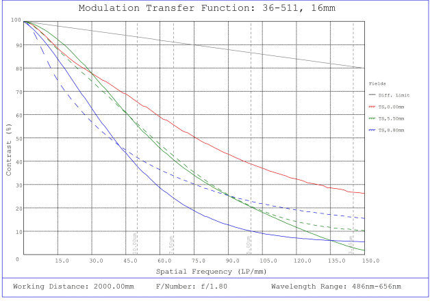
#36-511, 16mm f/1.8, HPr Series Fixed Focal Length Lens, Modulated Transfer Function (MTF) Plot, 2000mm Working Distance, f1.8
