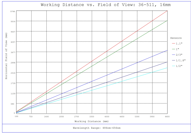
#36-511, 16mm f/1.8, HPr Series Fixed Focal Length Lens, Working Distance versus Field of View Plot
