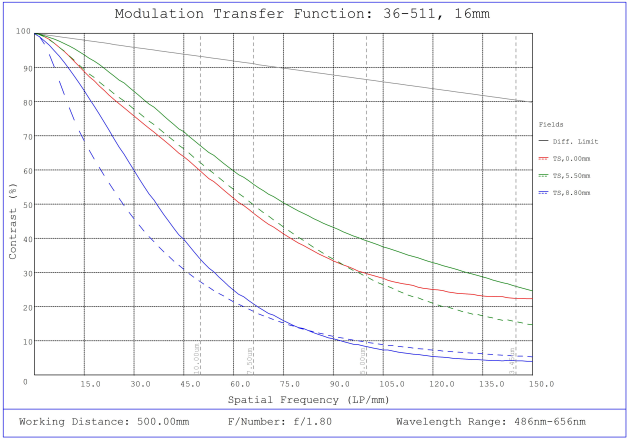
#36-511, 16mm f/1.8, HPr Series Fixed Focal Length Lens, Modulated Transfer Function (MTF) Plot, 500mm Working Distance, f1.8
