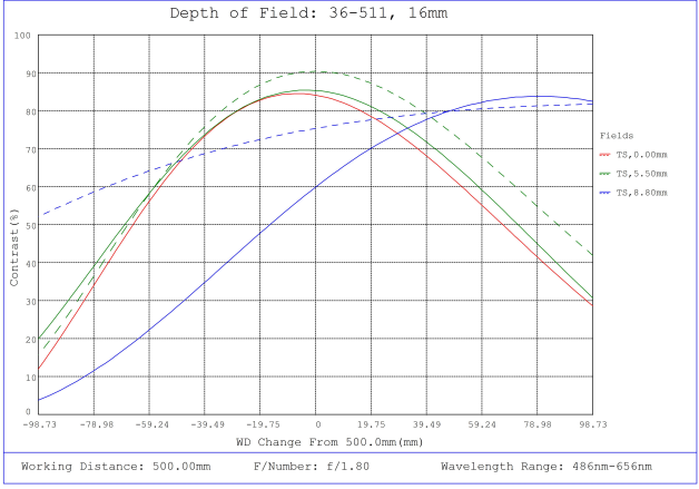
#36-511, 16mm f/1.8, HPr Series Fixed Focal Length Lens, Depth of Field Plot, 500mm Working Distance, f1.8
