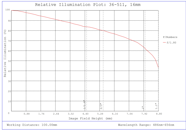
#36-511, 16mm f/1.8, HPr Series Fixed Focal Length Lens, Relative Illumination Plot
