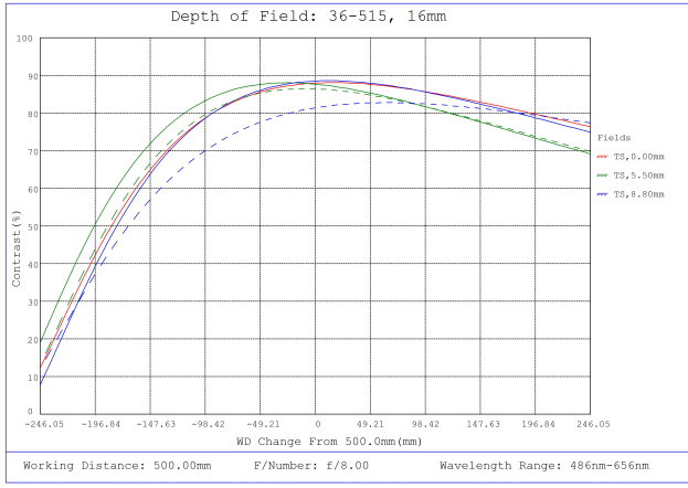
#36-515, 16mm f/8, HPr Series Fixed Focal Length Lens, Depth of Field Plot, 500mm Working Distance, f8
