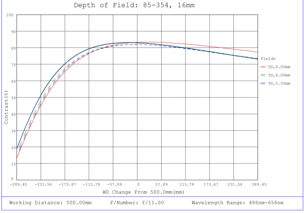
#85-354, 16mm, f/11 Ci Series Fixed Focal Length Lens, Depth of Field Plot, 500mm Working Distance, f11
