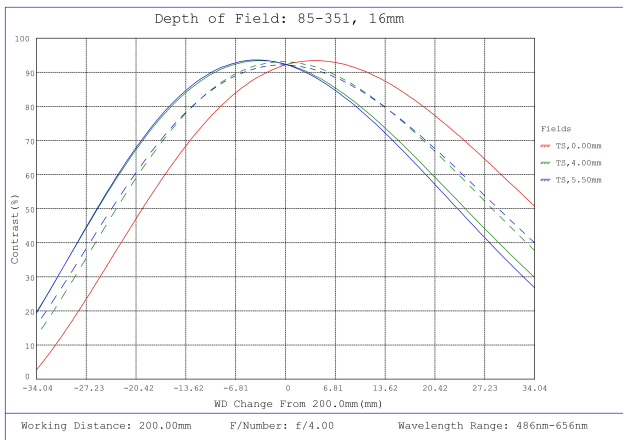
#85-351, 16mm, f/4 Ci Series Fixed Focal Length Lens, Depth of Field Plot, 200mm Working Distance, f4
