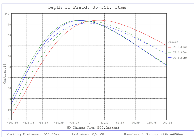
#85-351, 16mm, f/4 Ci Series Fixed Focal Length Lens, Depth of Field Plot, 500mm Working Distance, f4
