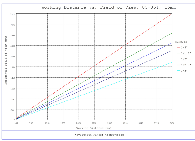
#85-351, 16mm, f/4 Ci Series Fixed Focal Length Lens, Working Distance versus Field of View Plot
