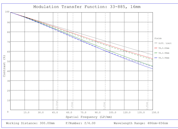
#33-885, 16mm, f/4 UCI Series Fixed Focal Length Lens, Modulated Transfer Function (MTF) Plot, 300mm Working Distance, f4
