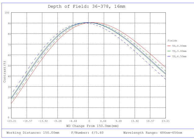
#36-378, 16mm FL f/5.6 Rugged Blue Series M12 Lens, Depth of Field Plot, 150mm Working Distance, f5.6
