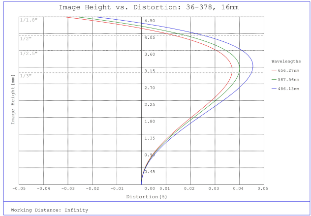
#36-378, 16mm FL f/5.6 Rugged Blue Series M12 Lens, Distortion Plot
