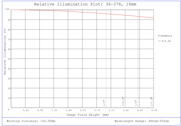
#36-378, 16mm FL f/5.6 Rugged Blue Series M12 Lens, Relative Illumination Plot
