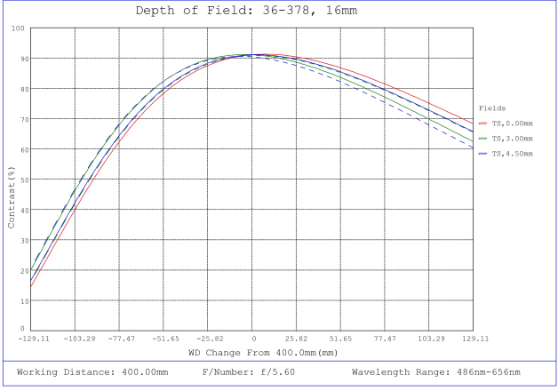
#36-378, 16mm FL f/5.6 Rugged Blue Series M12 Lens, Depth of Field Plot, 400mm Working Distance, f5.6
