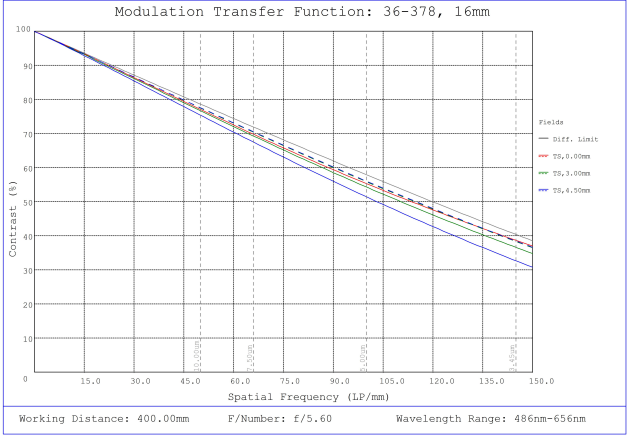
#36-378, 16mm FL f/5.6 Rugged Blue Series M12 Lens, Modulated Transfer Function (MTF) Plot, 400mm Working Distance, f5.6
