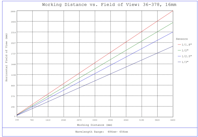
#36-378, 16mm FL f/5.6 Rugged Blue Series M12 Lens, Working Distance versus Field of View Plot
