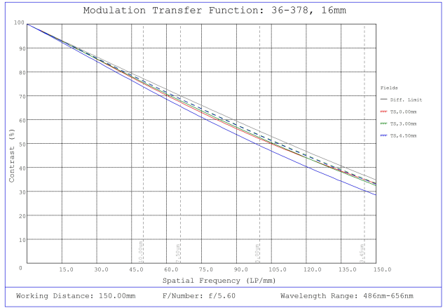
#36-378, 16mm FL f/5.6 Rugged Blue Series M12 Lens, Modulated Transfer Function (MTF) Plot, 150mm Working Distance, f5.6
