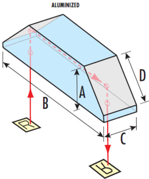
Displaced Retroreflector Ray Path
