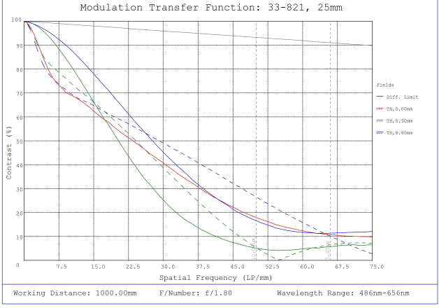
#33-821, 25mm f/1.8, HPi Series Fixed Focal Length Lens, Modulated Transfer Function (MTF) Plot, 1000mm Working Distance, f1.8
