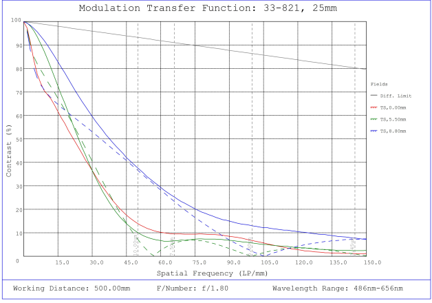
#33-821, 25mm f/1.8, HPi Series Fixed Focal Length Lens, Modulated Transfer Function (MTF) Plot, 500mm Working Distance, f1.8
