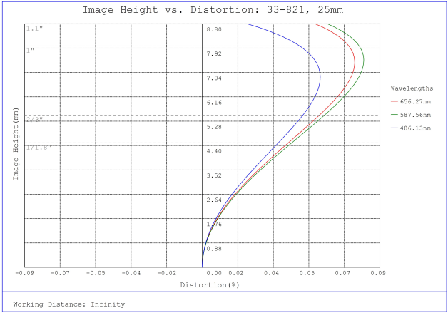
#33-821, 25mm f/1.8, HPI Series Fixed Focal Length Lens, Distortion Plot
