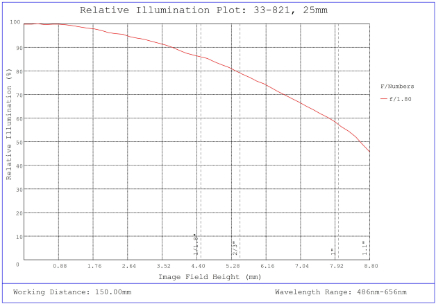
#33-821, 25mm f/1.8, HPI Series Fixed Focal Length Lens, Relative Illumination Plot
