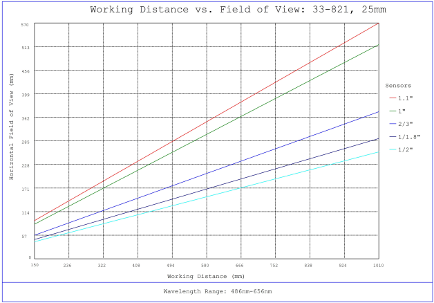
#33-821, 25mm f/1.8, HPI Series Fixed Focal Length Lens, Working Distance versus Field of View Plot
