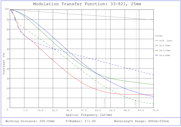
#33-821, 25mm f/1.8, HPi Series Fixed Focal Length Lens, Modulated Transfer Function (MTF) Plot, 200mm Working Distance, f1.8
