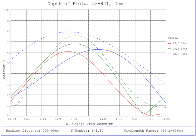
#33-821, 25mm f/1.8, HPi Series Fixed Focal Length Lens, Depth of Field Plot, 200mm Working Distance, f1.8
