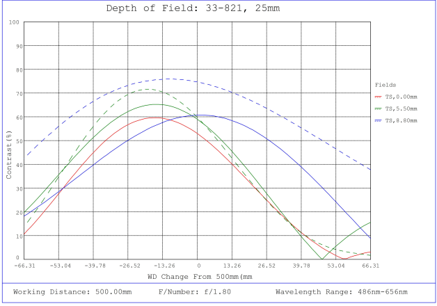
#33-821, 25mm f/1.8, HPi Series Fixed Focal Length Lens, Depth of Field Plot, 500mm Working Distance, f1.8
