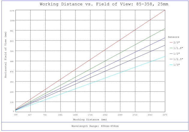
#85-358, 25mm, f/4 Ci Series Fixed Focal Length Lens, Working Distance versus Field of View Plot
