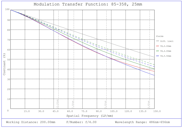
#85-358, 25mm, f/4 Ci Series Fixed Focal Length Lens, Modulated Transfer Function (MTF) Plot, 200mm Working Distance, f4
