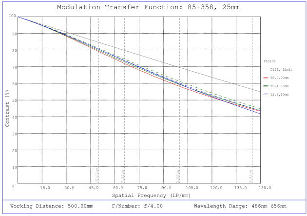
#85-358, 25mm, f/4 Ci Series Fixed Focal Length Lens, Modulated Transfer Function (MTF) Plot, 500mm Working Distance, f4
