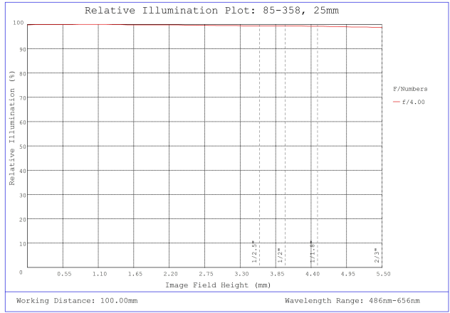
#85-358, 25mm, f/4 Ci Series Fixed Focal Length Lens, Relative Illumination Plot
