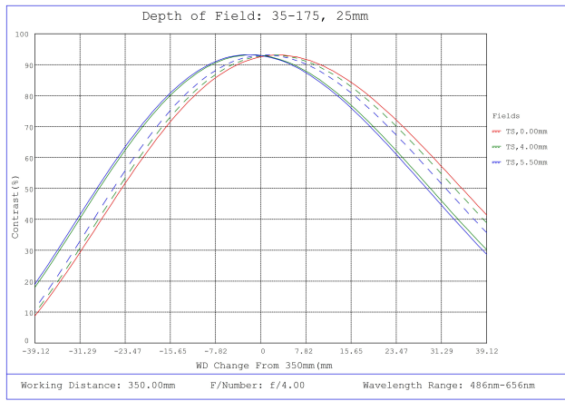
#35-175, 25mm, f/4 Cr Series Fixed Focal Length Lens, Depth of Field Plot, 350mm Working Distance, f4
