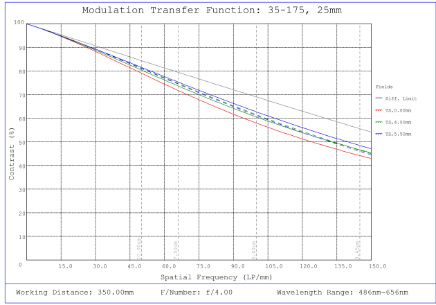
#35-175, 25mm, f/4 Cr Series Fixed Focal Length Lens, Modulated Transfer Function (MTF) Plot, 350mm Working Distance, f4
