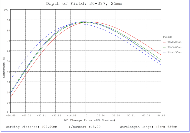
#36-387, 25mm FL f/8, Rugged Blue Series M12 Lens, Depth of Field Plot, 400mm Working Distance, f8
