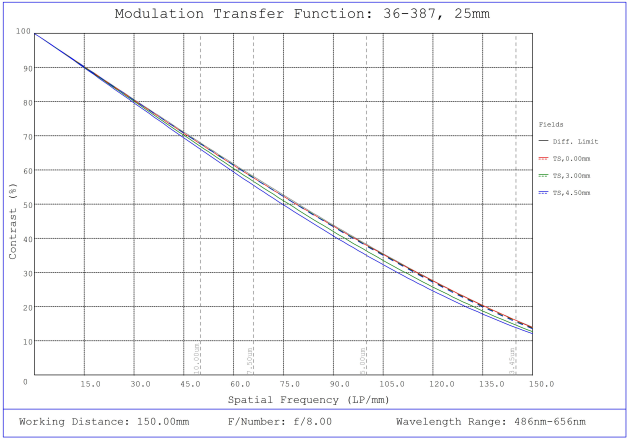
#36-387, 25mm FL f/8, Rugged Blue Series M12 Lens, Modulated Transfer Function (MTF) Plot, 150mm Working Distance, f8
