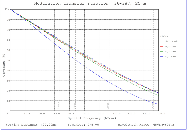
#36-387, 25mm FL f/8, Rugged Blue Series M12 Lens, Modulated Transfer Function (MTF) Plot, 400mm Working Distance, f8
