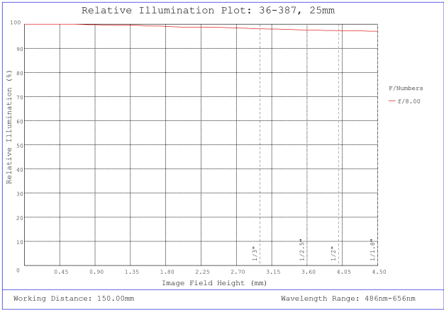
#36-387, 25mm FL f/8, Rugged Blue Series M12 Lens, Relative Illumination Plot
