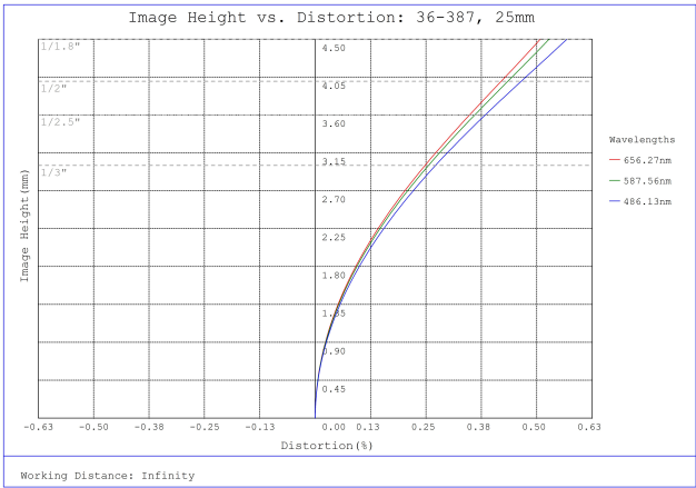
#36-387, 25mm FL f/8, Rugged Blue Series M12 Lens, Distortion Plot
