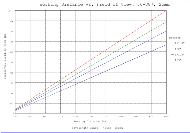
#36-387, 25mm FL f/8, Rugged Blue Series M12 Lens, Working Distance versus Field of View Plot
