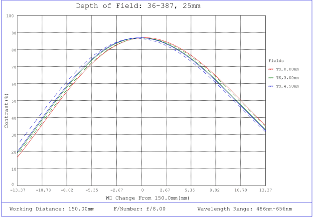
#36-387, 25mm FL f/8, Rugged Blue Series M12 Lens, Depth of Field Plot, 150mm Working Distance, f8
