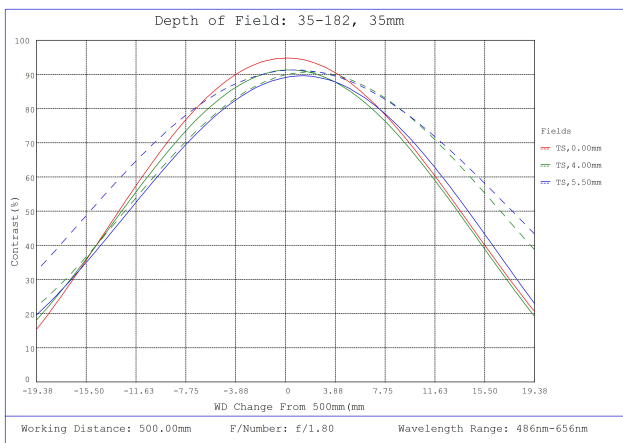
#35-182, 35mm, f/1.8 Cr Series Fixed Focal Length Lens, Depth of Field Plot, 500mm Working Distance, f1.8
