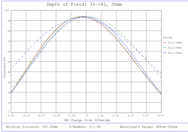
#35-182, 35mm, f/1.8 Cr Series Fixed Focal Length Lens, Depth of Field Plot, 300mm Working Distance, f1.8
