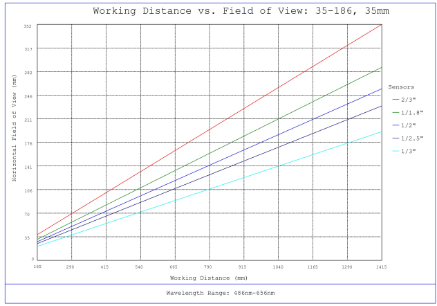
#35-186, 35mm, f/8.0 Cr Series Fixed Focal Length Lens, Working Distance versus Field of View Plot
