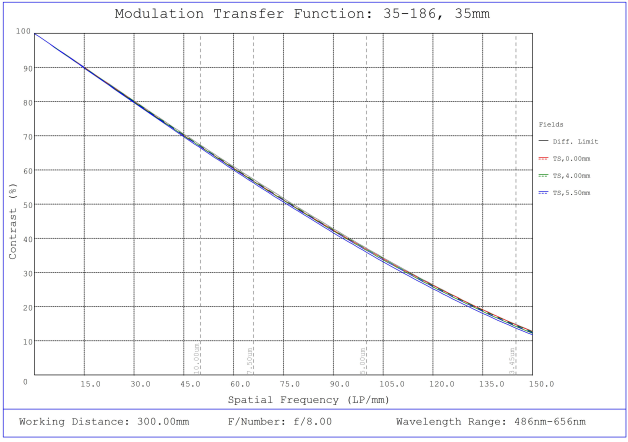
#35-186, 35mm, f/8.0 Cr Series Fixed Focal Length Lens, Modulated Transfer Function (MTF) Plot, 300mm Working Distance, f8
