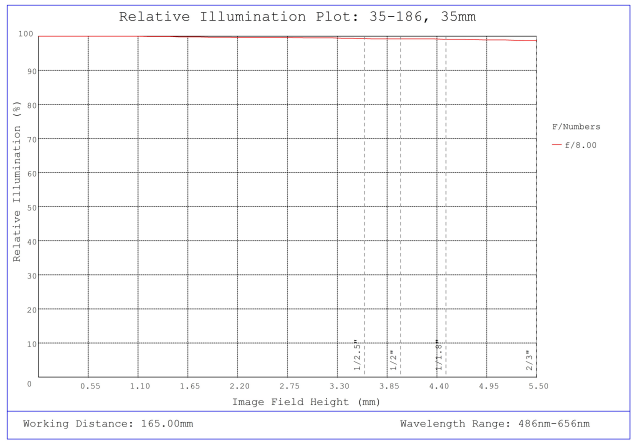
#35-186, 35mm, f/8.0 Cr Series Fixed Focal Length Lens, Relative Illumination Plot
