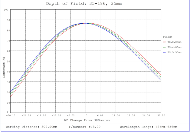
#35-186, 35mm, f/8.0 Cr Series Fixed Focal Length Lens, Depth of Field Plot, 300mm Working Distance, f8
