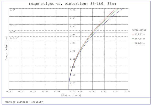
#35-186, 35mm, f/8.0 Cr Series Fixed Focal Length Lens, Distortion Plot
