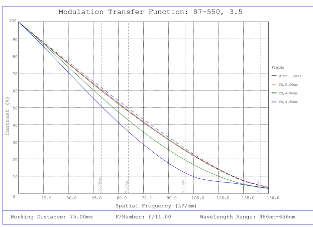
#87-550, 3.5mm, f/11 Ci Series Fixed Focal Length Lens, Modulated Transfer Function (MTF) Plot, 75mm Working Distance, f11
