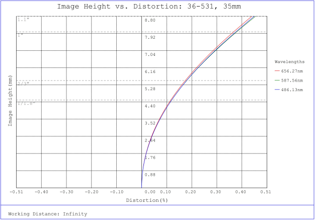
#36-531, 35mm f/11.0, HPr Series Fixed Focal Length Lens, Distortion Plot
