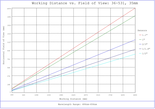
#36-531, 35mm f/11.0, HPr Series Fixed Focal Length Lens, Working Distance versus Field of View Plot
