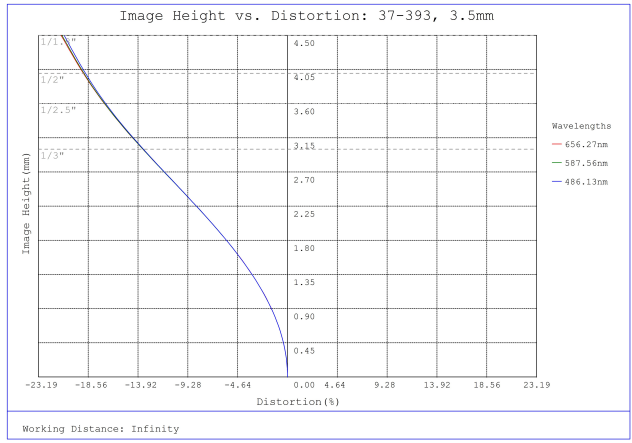
#37-393, 3.5mm, f/2.8 Cr Series Fixed Focal Length Lens, Distortion Plot
