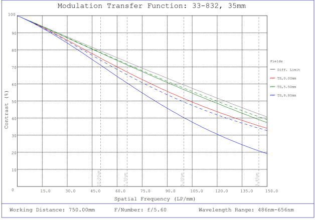
#33-832, 35mm f/5.6, HPi Series Fixed Focal Length Lens, Modulated Transfer Function (MTF) Plot, 750mm Working Distance, f5.6
