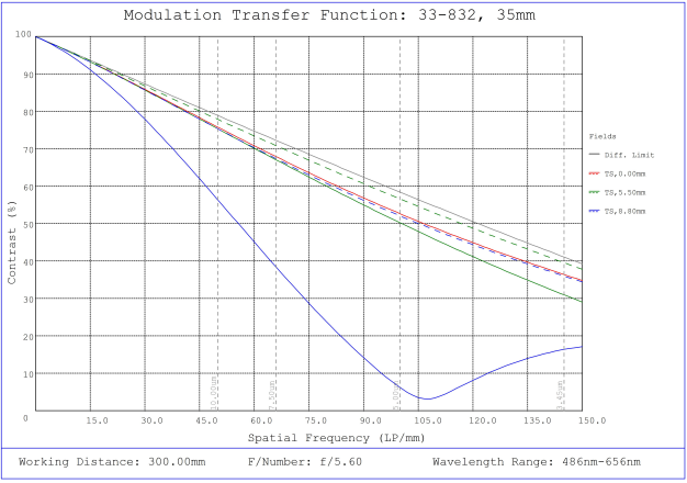
#33-832, 35mm f/5.6, HPI Series Fixed Focal Length Lens, Modulated Transfer Function (MTF) Plot, 300mm Working Distance, f5.6
