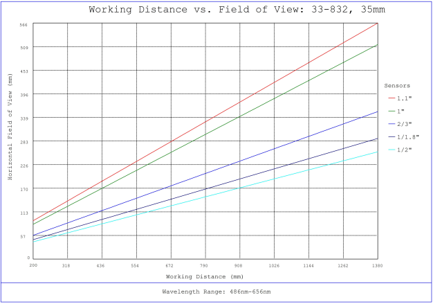
#33-832, 35mm f/5.6, HPI Series Fixed Focal Length Lens, Working Distance versus Field of View Plot
