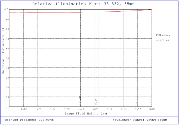
#33-832, 35mm f/5.6, HPI Series Fixed Focal Length Lens, Relative Illumination Plot
