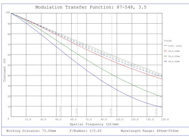
#87-548, 3.5mm, f/5.6 Ci Series Fixed Focal Length Lens, Modulated Transfer Function (MTF) Plot, 75mm Working Distance, f5.6
