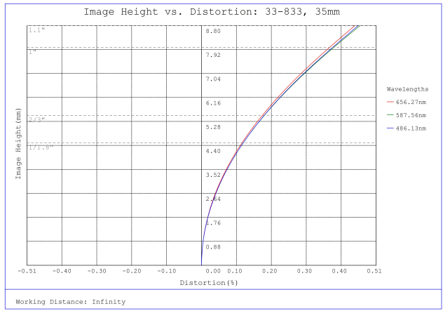
#33-833, 35mm f/8.0, HPi Series Fixed Focal Length Lens, Distortion Plot
