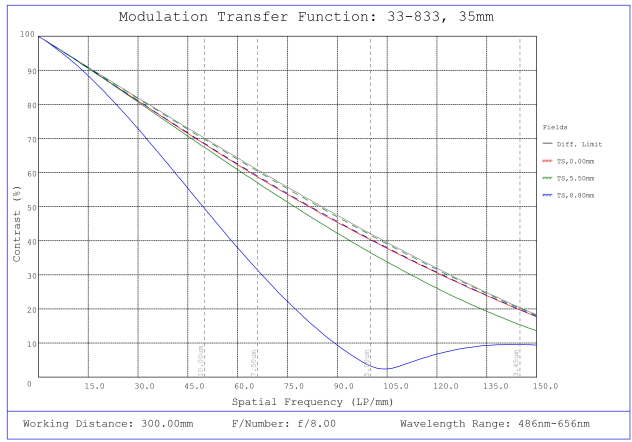
#33-833, 35mm f/8.0, HPi Series Fixed Focal Length Lens, Modulated Transfer Function (MTF) Plot, 300mm Working Distance, f8
