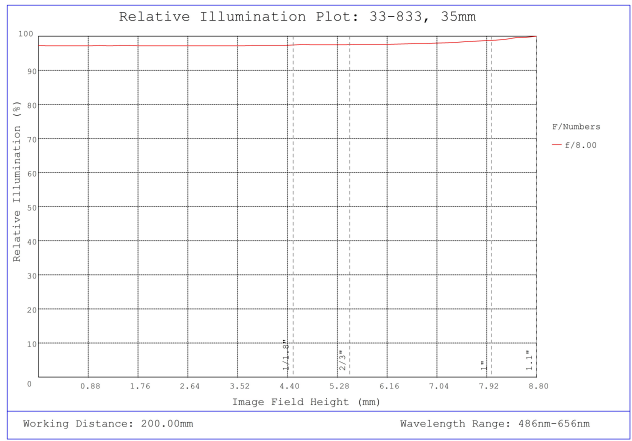
#33-833, 35mm f/8.0, HPi Series Fixed Focal Length Lens, Relative Illumination Plot
