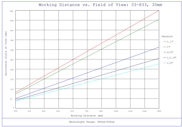
#33-833, 35mm f/8.0, HPi Series Fixed Focal Length Lens, Working Distance versus Field of View Plot
