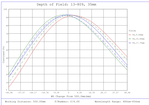
#13-809, 35mm TFL-II Mount LH Series Fixed Focal Length Lens, Depth of Field Plot, 500mm Working Distance, f4
