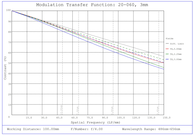
#20-060, 3mm FL f/4.0 IR-Cut Rugged Blue Series M12 Lens, Modulated Transfer Function (MTF) Plot, 100mm Working Distance, f4
