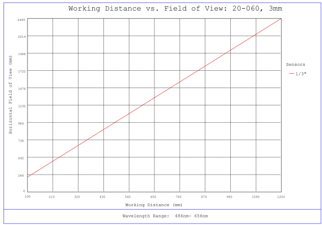
#20-060, 3mm FL f/4.0 IR-Cut Rugged Blue Series M12 Lens, Working Distance versus Field of View Plot
