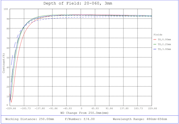
#20-060, 3mm FL f/4.0 IR-Cut Rugged Blue Series M12 Lens, Depth of Field Plot, 250mm Working Distance, f4
