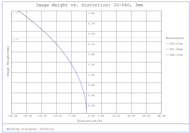
#20-060, 3mm FL f/4.0 IR-Cut Rugged Blue Series M12 Lens, Distortion Plot
