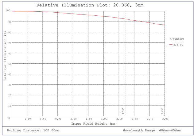
#20-060, 3mm FL f/4.0 IR-Cut Rugged Blue Series M12 Lens, Relative Illumination Plot
