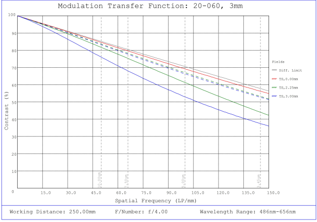
#20-060, 3mm FL f/4.0 IR-Cut Rugged Blue Series M12 Lens, Modulated Transfer Function (MTF) Plot, 250mm Working Distance, f4
