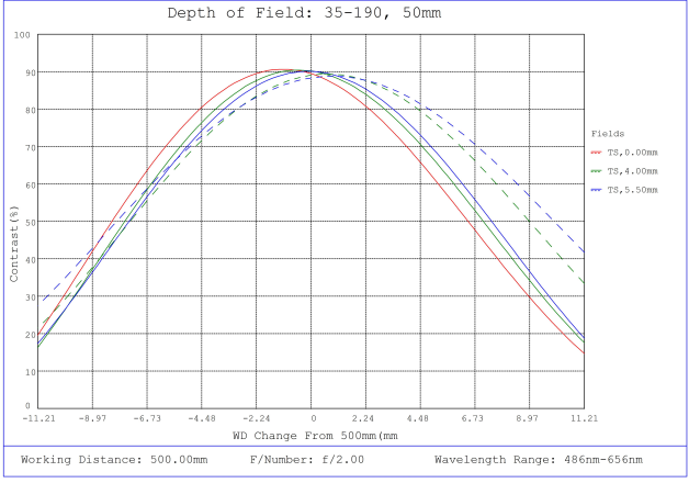
#35-190, 50mm, f/2.0 Cr Series Fixed Focal Length Lens, Depth of Field Plot, 500mm Working Distance, f2
