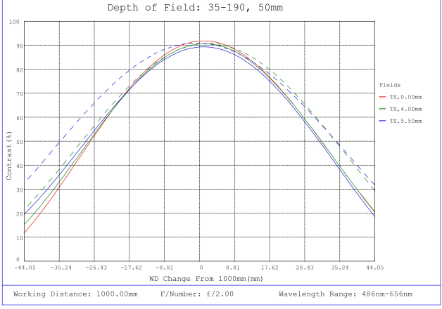
#35-190, 50mm, f/2.0 Cr Series Fixed Focal Length Lens, Depth of Field Plot, 1000mm Working Distance, f2
