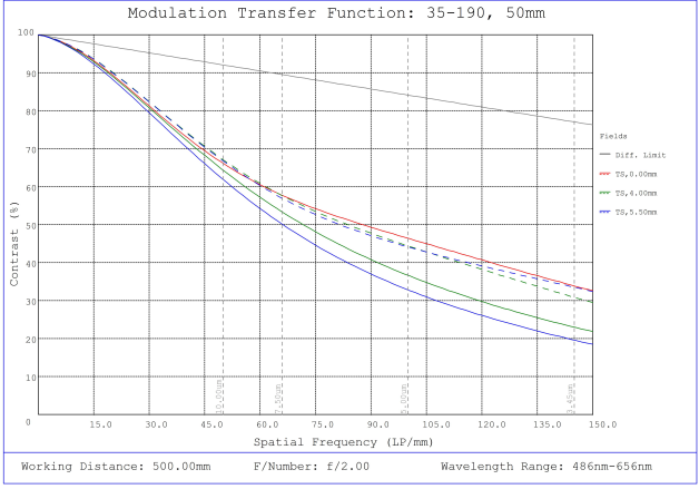
#35-190, 50mm, f/2.0 Cr Series Fixed Focal Length Lens, Modulated Transfer Function (MTF) Plot, 500mm Working Distance, f2
