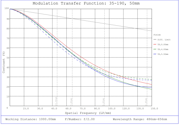
#35-190, 50mm, f/2.0 Cr Series Fixed Focal Length Lens, Modulated Transfer Function (MTF) Plot, 1000mm Working Distance, f2
