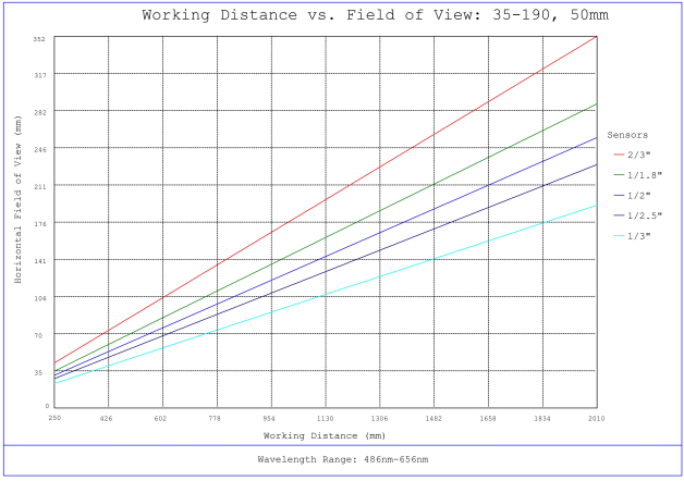
#35-190, 50mm, f/2.0 Cr Series Fixed Focal Length Lens, Working Distance versus Field of View Plot
