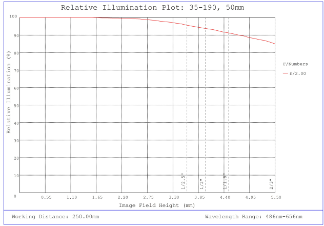
#35-190, 50mm, f/2.0 Cr Series Fixed Focal Length Lens, Relative Illumination Plot
