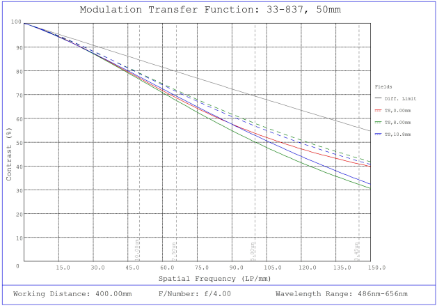
#33-837, 50mm f/4.0, HPi Series Fixed Focal Length Lens, Modulated Transfer Function (MTF) Plot, 400mm Working Distance, f4
