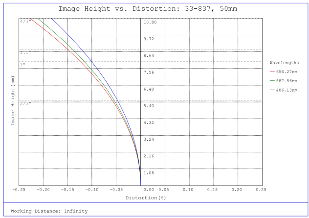
#33-837, 50mm f/4.0, HPI Series Fixed Focal Length Lens, Distortion Plot
