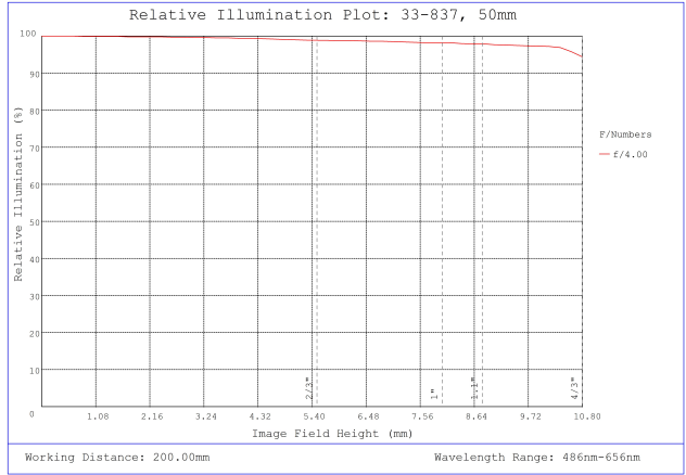
#33-837, 50mm f/4.0, HPI Series Fixed Focal Length Lens, Relative Illumination Plot
