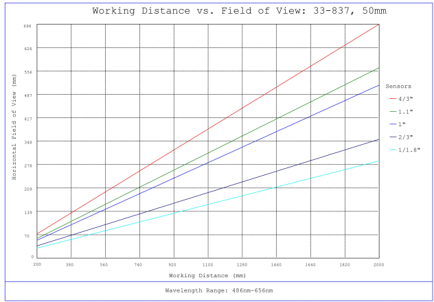
#33-837, 50mm f/4.0, HPI Series Fixed Focal Length Lens, Working Distance versus Field of View Plot
