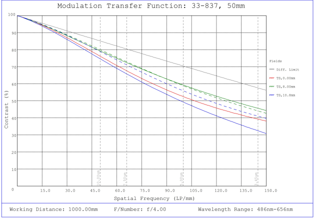
#33-837, 50mm f/4.0, HPi Series Fixed Focal Length Lens, Modulated Transfer Function (MTF) Plot, 1000mm Working Distance, f4
